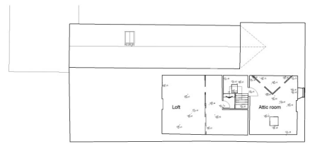
Second Floor Plan 1:100
